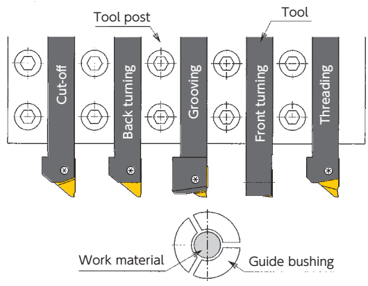
Tooling for gang type tool post
