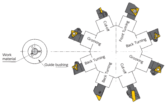
Tooling for turret type tool post
